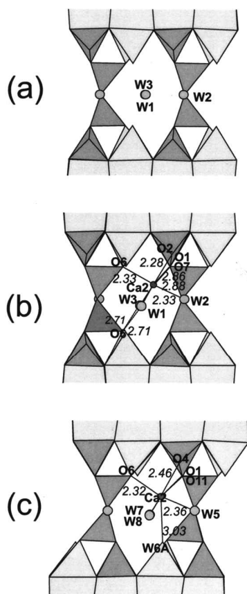
Fig. 9. Schematic drawing of the structural cavities, as seen along [010] in (a) anomalous tobermorite 11Å from Wessels mine; (b) normal tobermorite 11Å from Urals; (c) clinotobermorite from Wessels mine (Merlino et al. , 2000). In (b) one of the two possible ordered arrangements of Ca2, W1, and W3 is reported.
