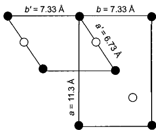
Fig. 3. Relationships between the C centred cell, which presents additional lattice points at 1/4 , 1/4 , 1/2 (empty circles), and the B centred cell of the \text{MDO}_2 polytype of tobermorite 11Å.
