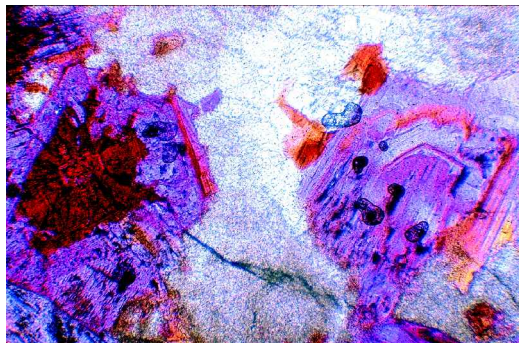
FIG. 1. Thin-section of strongly zoned manganovesuvianite in a grossular matrix (sample NC14). The dark red vesuvianite cores typically contain 6–9 wt.% MnO, lilac zones contain 1.5–5 wt.% MnO. Base of photograph is 1 mm long; plane polarized light.
