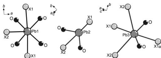
Fig. 2. Coordination of \text{Pb} atoms in the structures of the mendipite series \text{Pb}_3\text{O}_2\text{Cl}_2\text{--Pb}_3\text{O}_2\text{Br}_2 .
